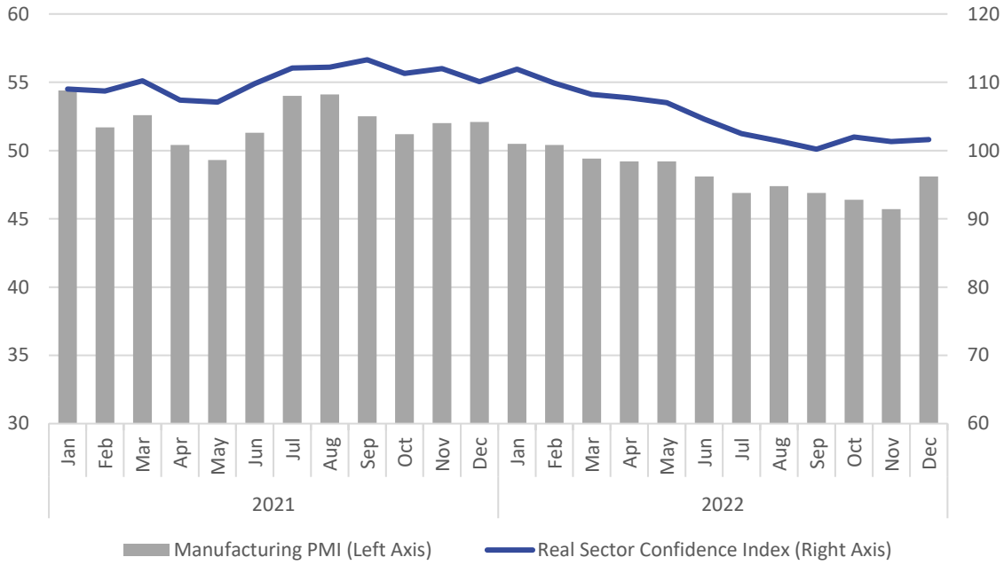
Figure 3: Manufacturing Purchasing Managers' Index vs. Real Sector Confidence Index
